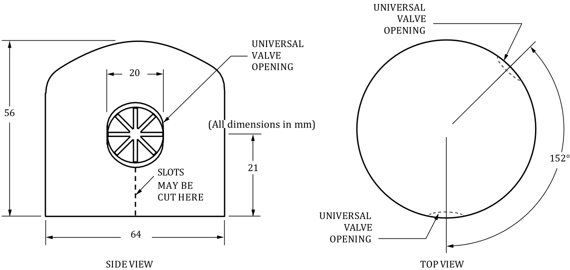
Figure 11. Universal wildlife protector for line terminal adds 5 mm to arrester height above line terminal stud. To be used only with 10 mm or 12 mm Ø line hardware of standard length, 30 mm.
