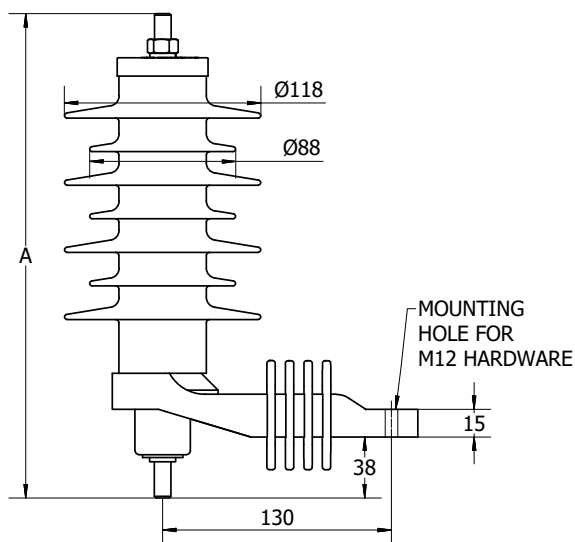
Figure 4. Polymer-housed surge arrester— with optional insulated mounting bracket and disconnector
