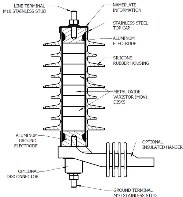
Figure 1. Cutaway illustration of a molded polymer-housed surge arrester
