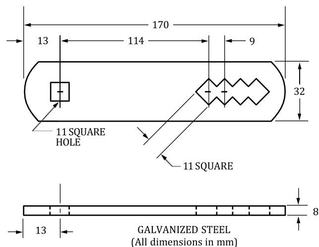
Figure 9. Conductive base mounting for use with 3/8 inch hardware. Can be specified with a “2” in digit 12. (Requires “A”, “B” or “C” in digit 10, “D” in digit 11)
