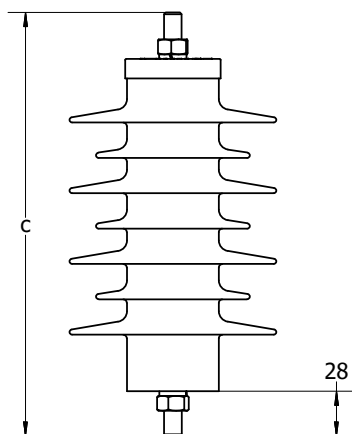
Figure 5. Polymer-housed surge arrester without disconnector, for base or cable riser mounting (arrester may be horizontal or vertical with either end at line potential)
