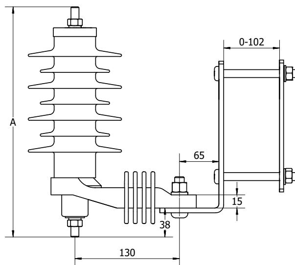
Figure 6. Polymer-housed surge arrester as in Figure 4 with NEMA cross-arm hanger, see Figure 8
