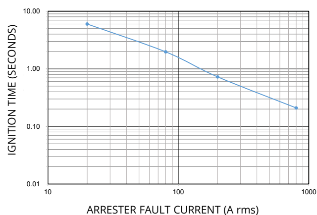
Figure 2. MHD disconnector operating characteristics
