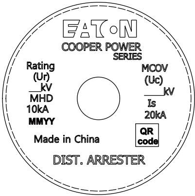
Figure 12. I_n = 10 kA, Class DH, nameplate—stamped in stainless steel top cap
