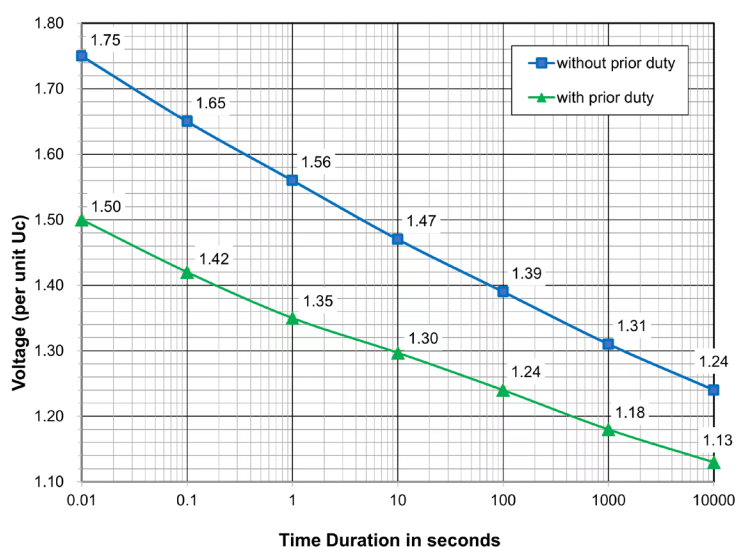
Figure 3. Temporary overvoltage capability
