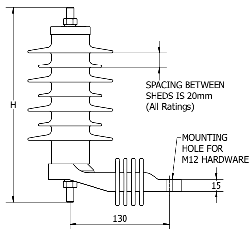
Figure 7. Polymer-housed surge arrester—with optional disconnector mounting bracket (no disconnector)
