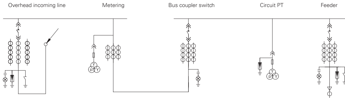
Typical primary scheme diagram
