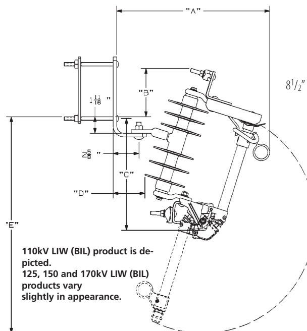
STANDARD Type C-Polymer Cutout with NEMA Type B Bracket
